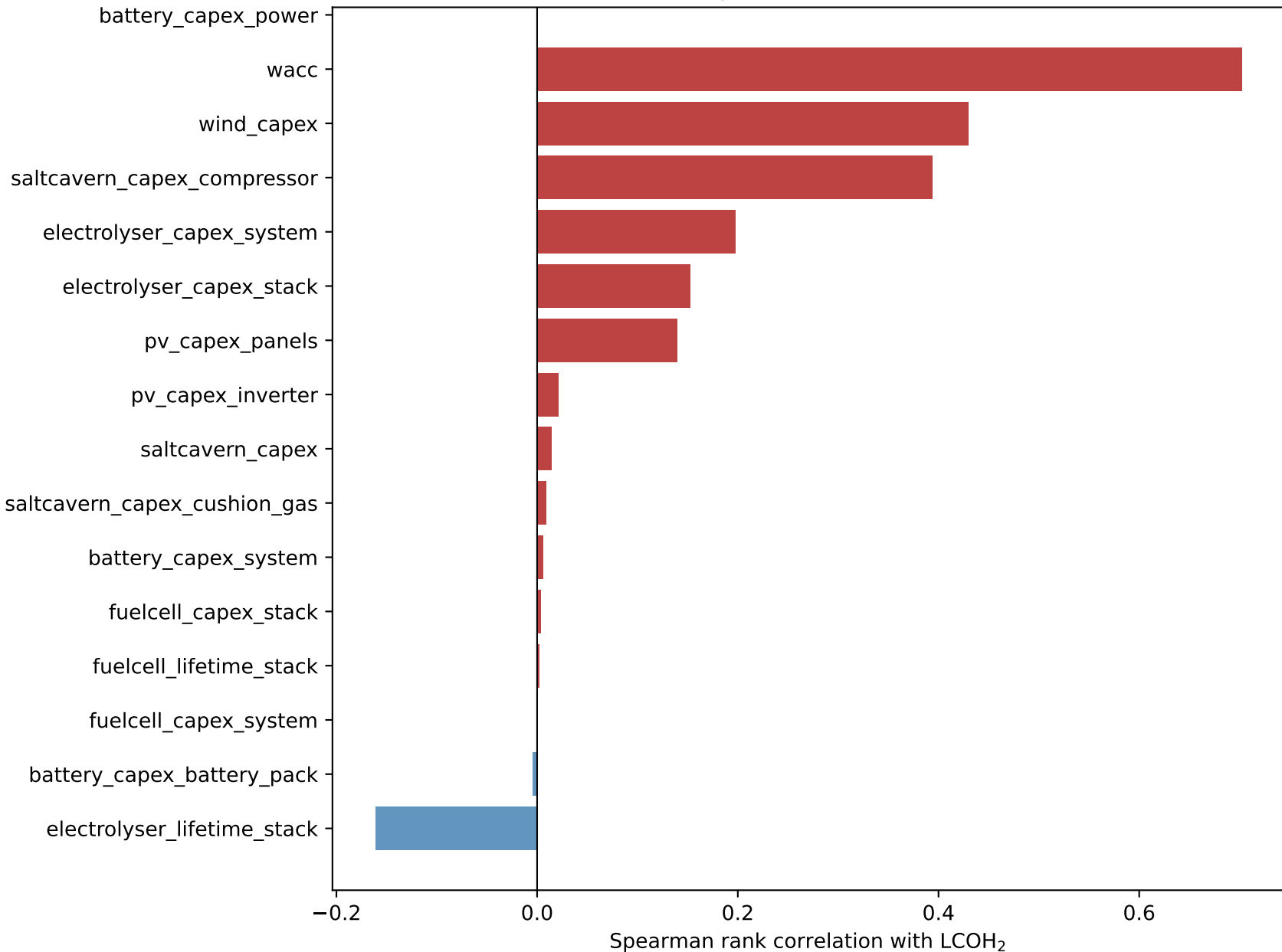
CAPEX Sensitivity — Tornado Plot (N=100,000)
